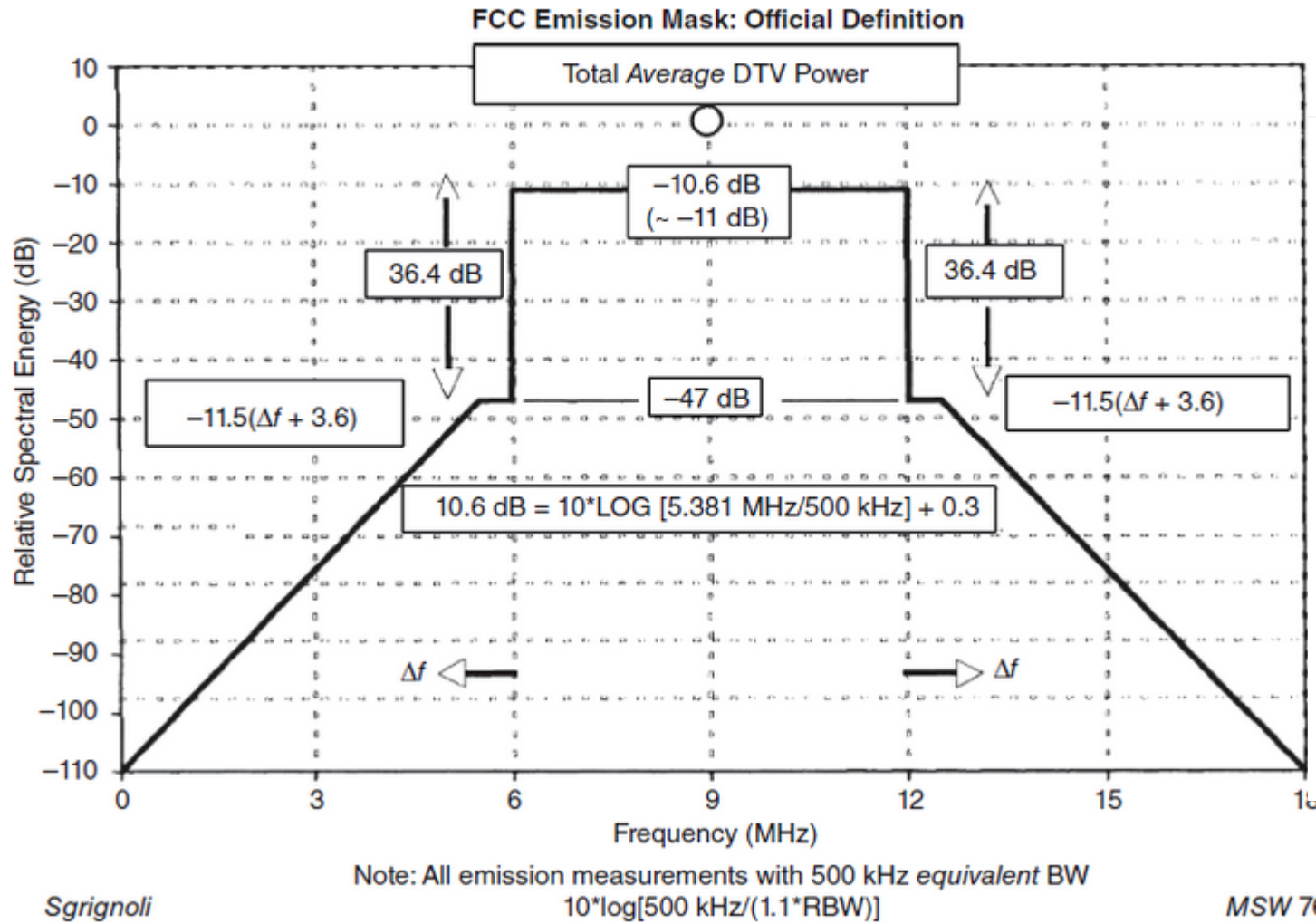
Figure 1.8.10 FCC spectral mask for 8-VSB transmitters. (Courtesy: Meintel Sgrignoli Wallace.)
