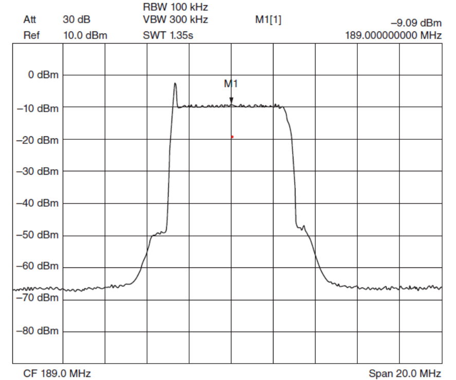
Figure 1.8.11 8-VSB spectral display.
